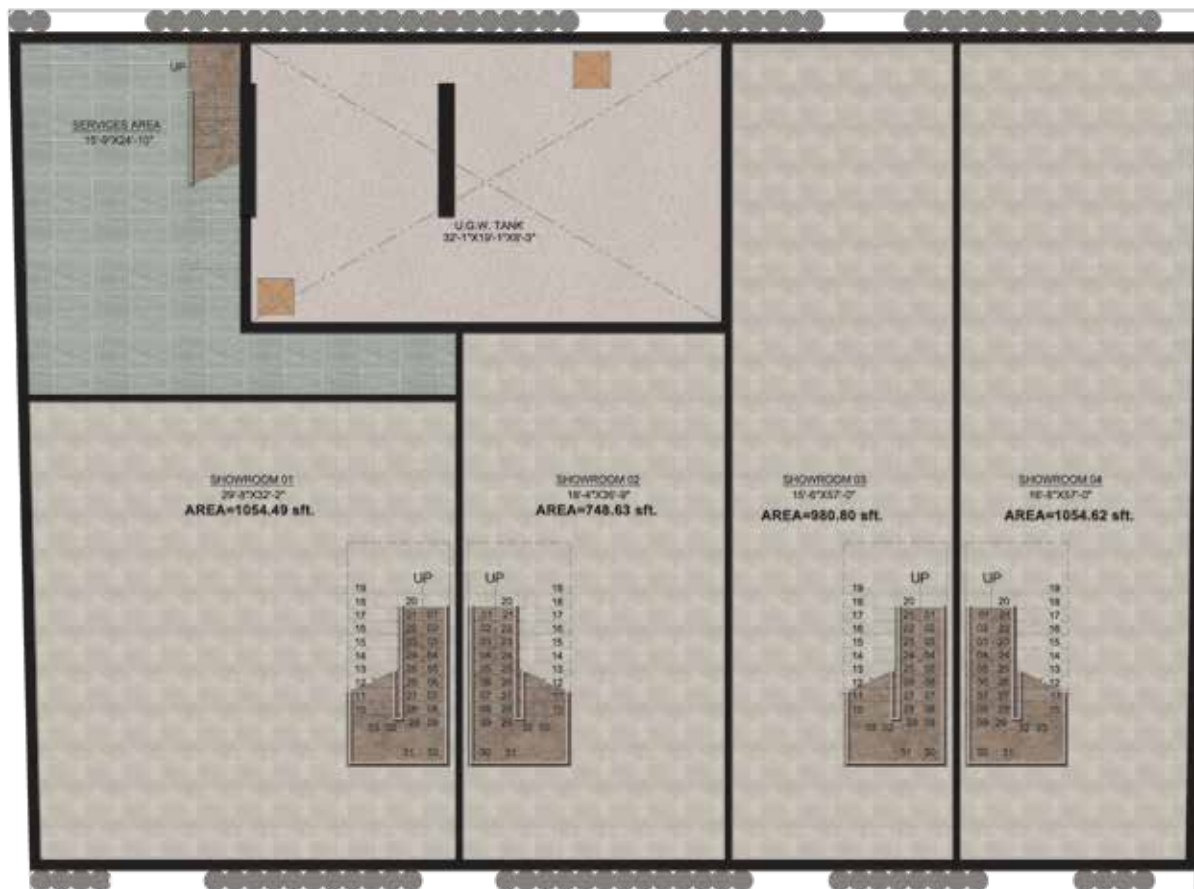
BASEMENT FLOOR PLAN (AT LEVEL -15'-9")
